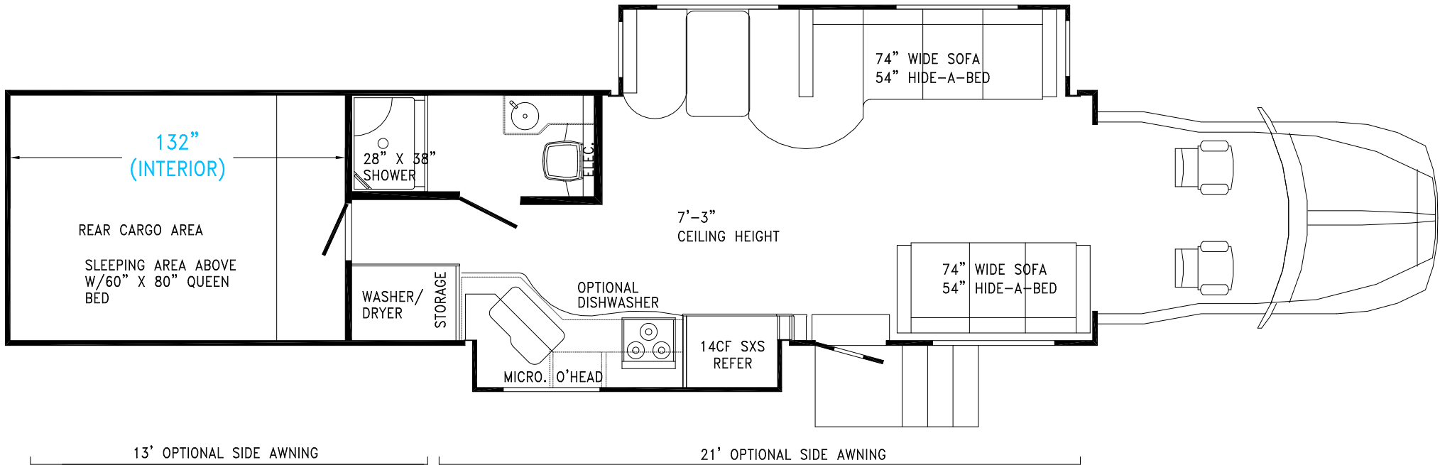
2008 - 47' GARAGE UNIT DAY CAB
